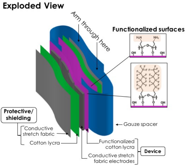
Figure 4: Physical Structure of the Tribexor joint sensor
